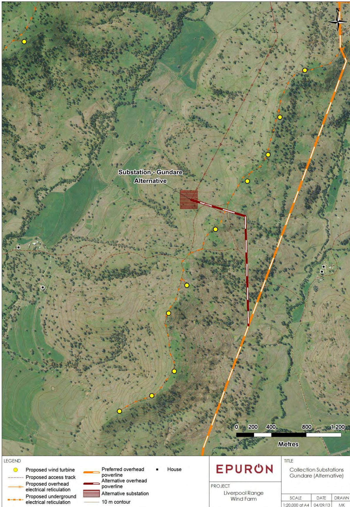
Figure 30 Detailed view of the alternative Gundare substation
